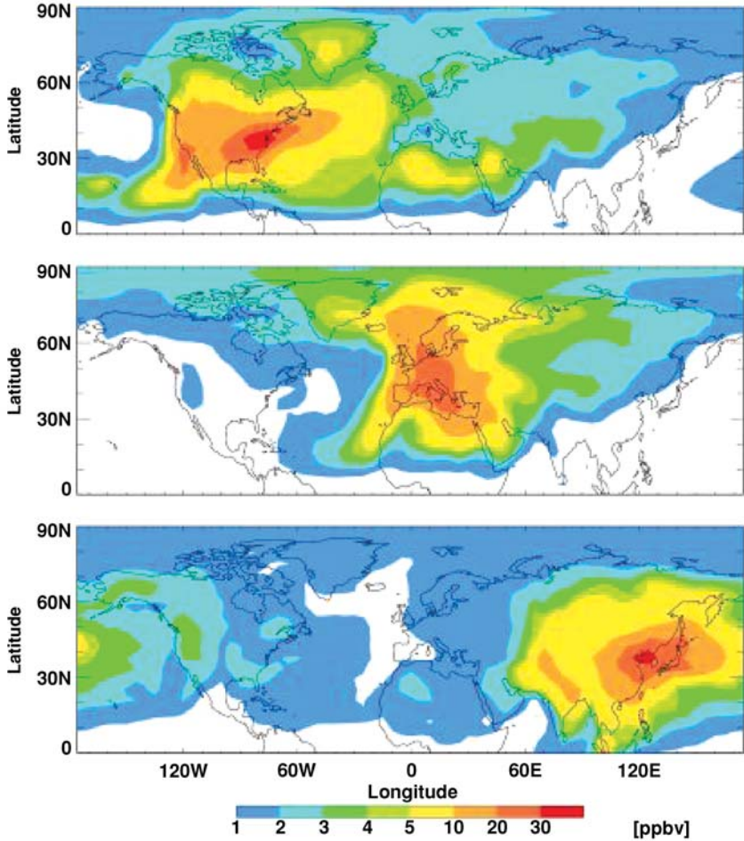
Figure 7 Model estimates of surface ozone attributable to anthropogenic emissions from North America ( top panel ), Europe ( middle panel ), and Asia ( lower panel ) during June, July, and August 1997. Units are in parts per billion volume (ppbv). [From (71).]
